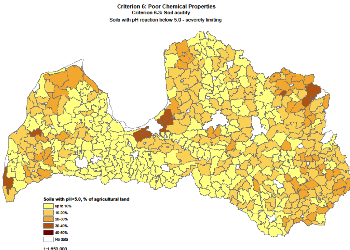
Figure 3.6-1: Simulation results of the Criteria 6: Poor chemical properties – Soil Acidity
