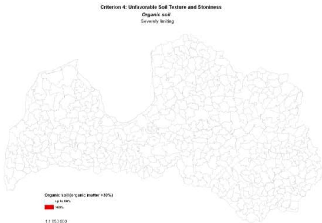
Figure 3.4-5: Criterion “SOIL TEXTURE AND STONINESS” – organic soils. Areas considered as affected by significant natural handicaps with >60% compliance
