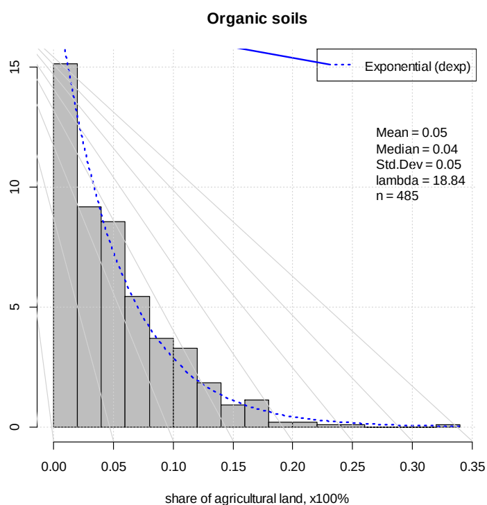
Figure 3.4-6: Criterion “SOIL TEXTURE AND STONINESS: organic soils” the share of organic soils in agricultural lands in Latvia.
