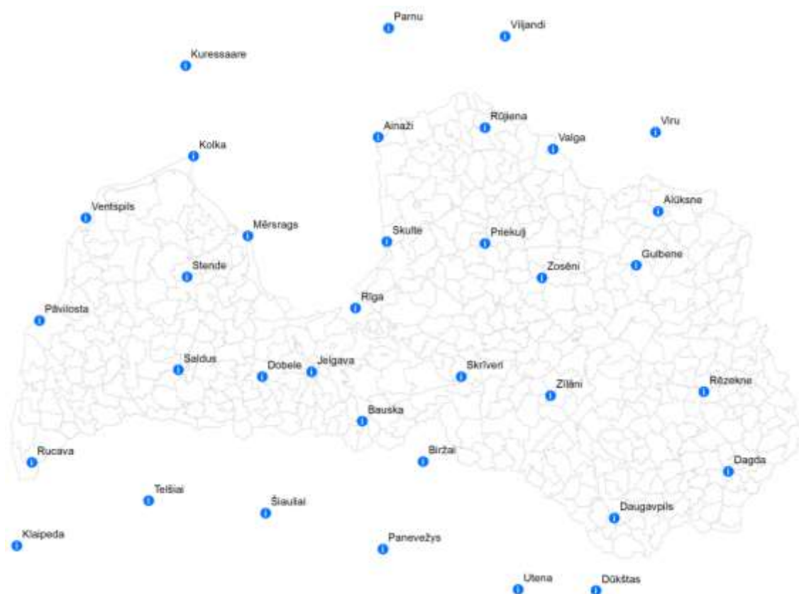
Figure 2.1-1: Meteorological stations in Latvia, Lithuania and Estonia used in delineation of climate ANC territories in Latvia, including stations in Estonia and Lithuania used in delineation of ANC territories in Latvia.
