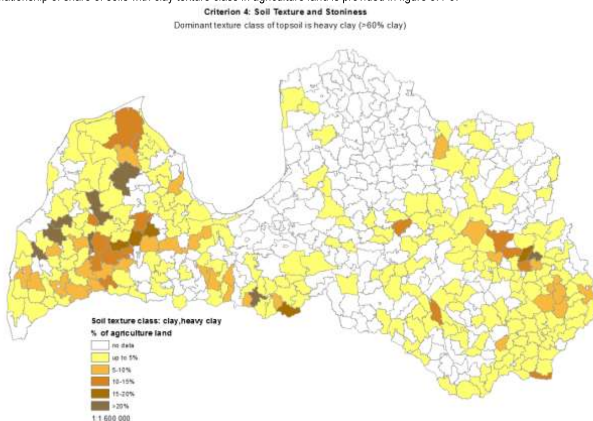
Figure 3.4-7: Overall situation in Latvia: Simulation results of the Criterion “SOIL TEXTURE AND STONINESS” – organic soils
