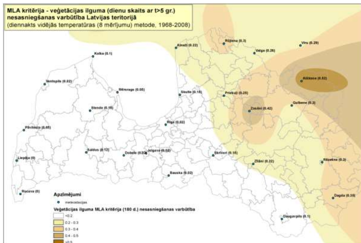
Figure 3.1-1: : Delineation of ANC criterion: Length of the Temperature Growing Period occurrence probabilities (8 measurement method, data range 1968-2008).
