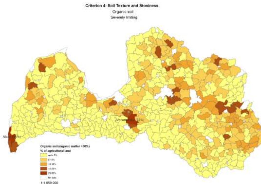
Figure 3.4-4: Overall situation in Latvia: Simulation results of the Criterion "SOIL TEXTURE AND STONINESS" – organic soils
