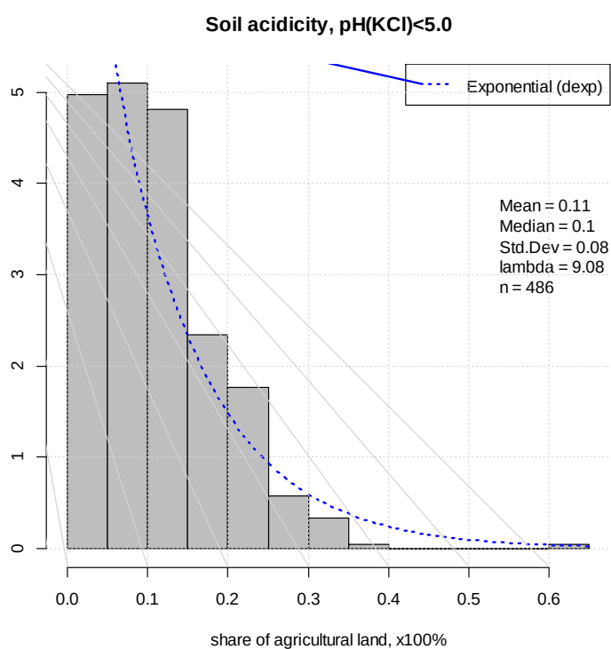
Figure 3.6-3: Criterion “6. Poor chemical properties: 6.3 Soil acidity”: the share of soils with pH<5.0 in agricultural lands in Latvia.
