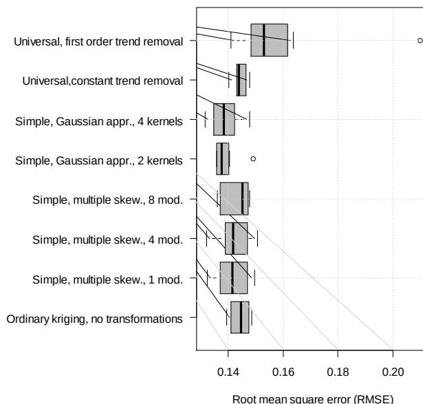
Figure 3.1-7: Comparison of tested co-kriging interpolation method and semivariogram models
