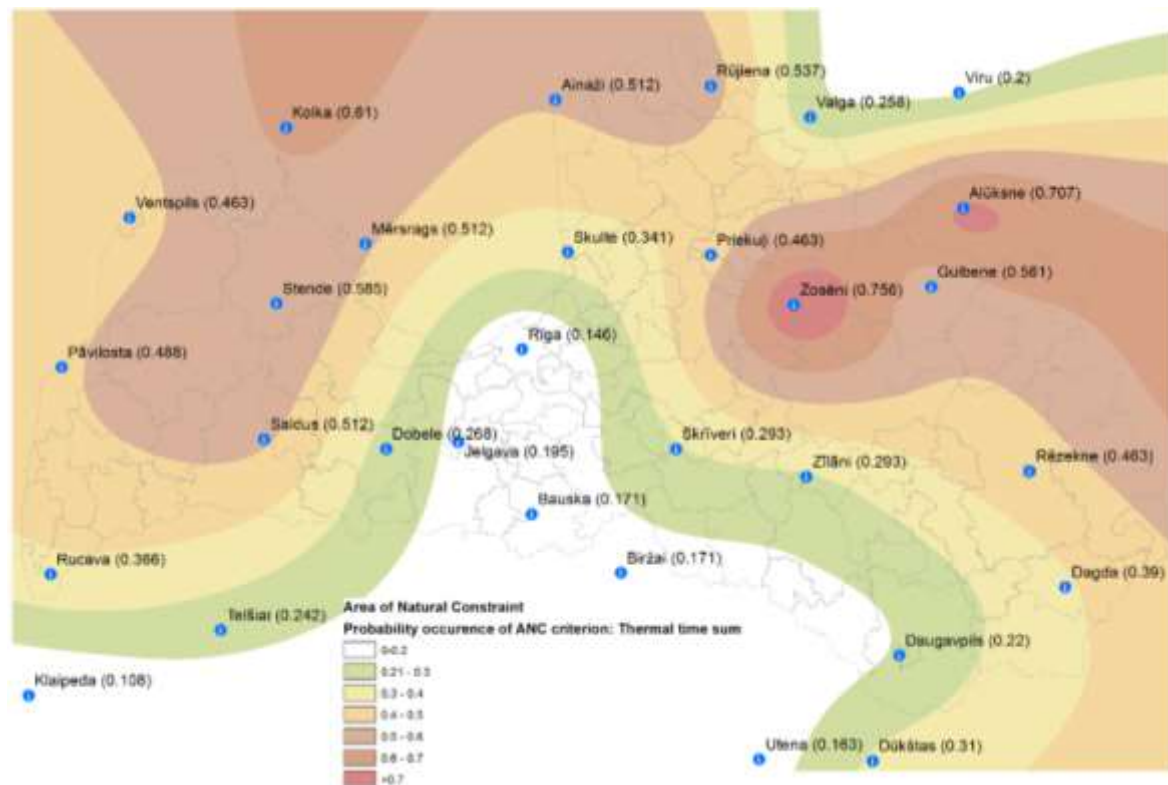
Figure 3.1-5: Territories where ANC criterion thermal-time sum ANC criterion occurrence possibility exceeds 20% (8 measurement method, period 1968-2008). Liepāja meteorostation excluded from the climate data set as described above.
