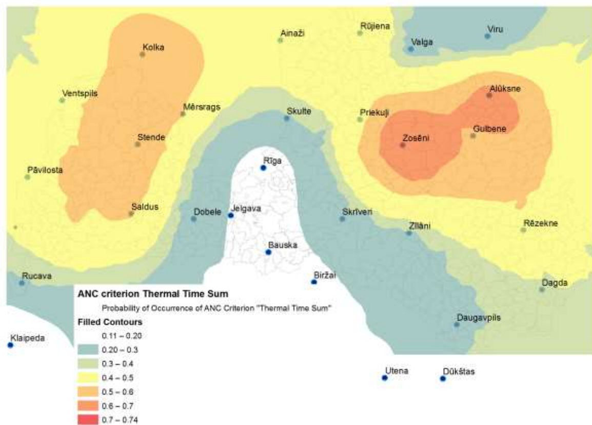
Figure 3.1-11: Refined delineation of ANC territories where the Thermal Time Sum criterion occurrence probability exceeds 20% (8 measurement method, period 1968-2008) using co-kriging interpolation method
