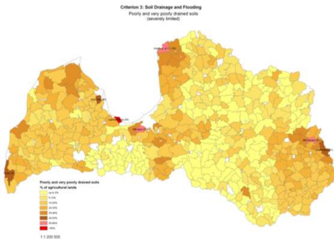
Figure 3.3-3: Overall situation in Latvia: Simulation results of the Criterion “DRAINAGE” – Poorly and very poorly drained soils
