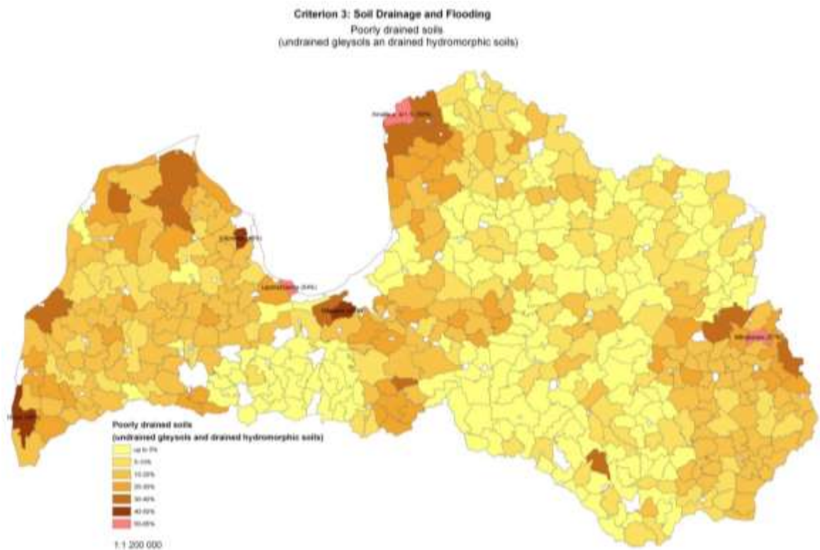
Figure 3.3-4: Overall situation in Latvia: Simulation results of the Criterion “DRAINAGE” – Poorly drained soils
