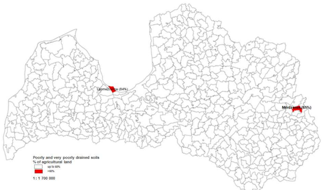
Figure 3.3-5: Criterion “DRAINAGE”. Poorly drained and very poorly drained soils – Areas considered as affected by significant natural handicaps with >60% compliance
