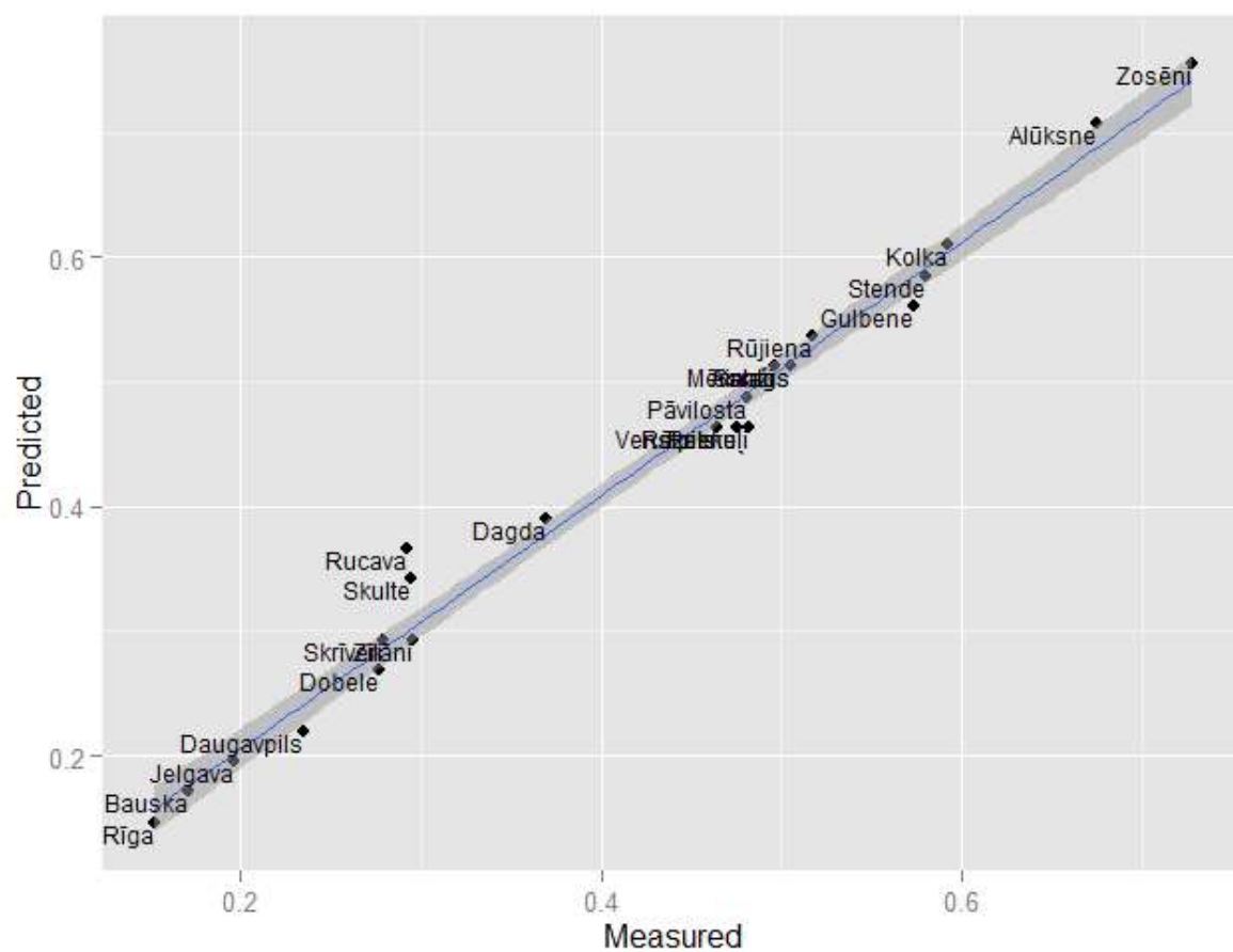
Figure 3.1-8: Simple co-kriging interpolation method cross-validation: measured ANC probability values vs predicted ANC probability values. Linear regression model, 95% confidence interval. Statistics: Pearson r=0.992 , r^2= 0.984 , p= 0.027 .
