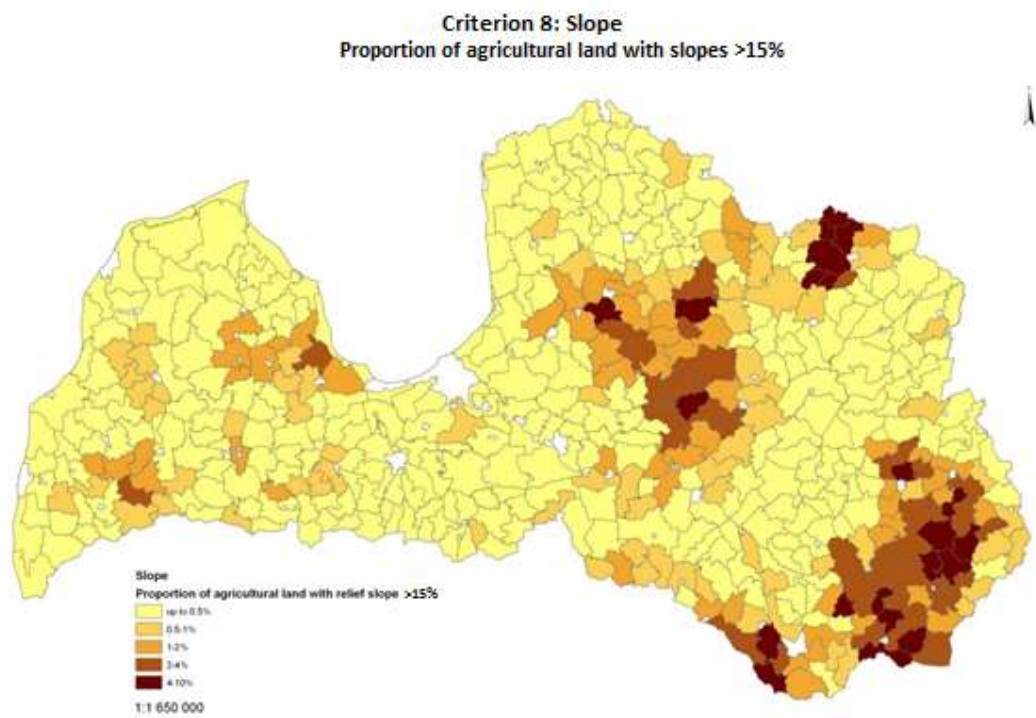
Figure 3.8-1: Simulation results of the Criterion “Slope” (based on digital elevation model)
