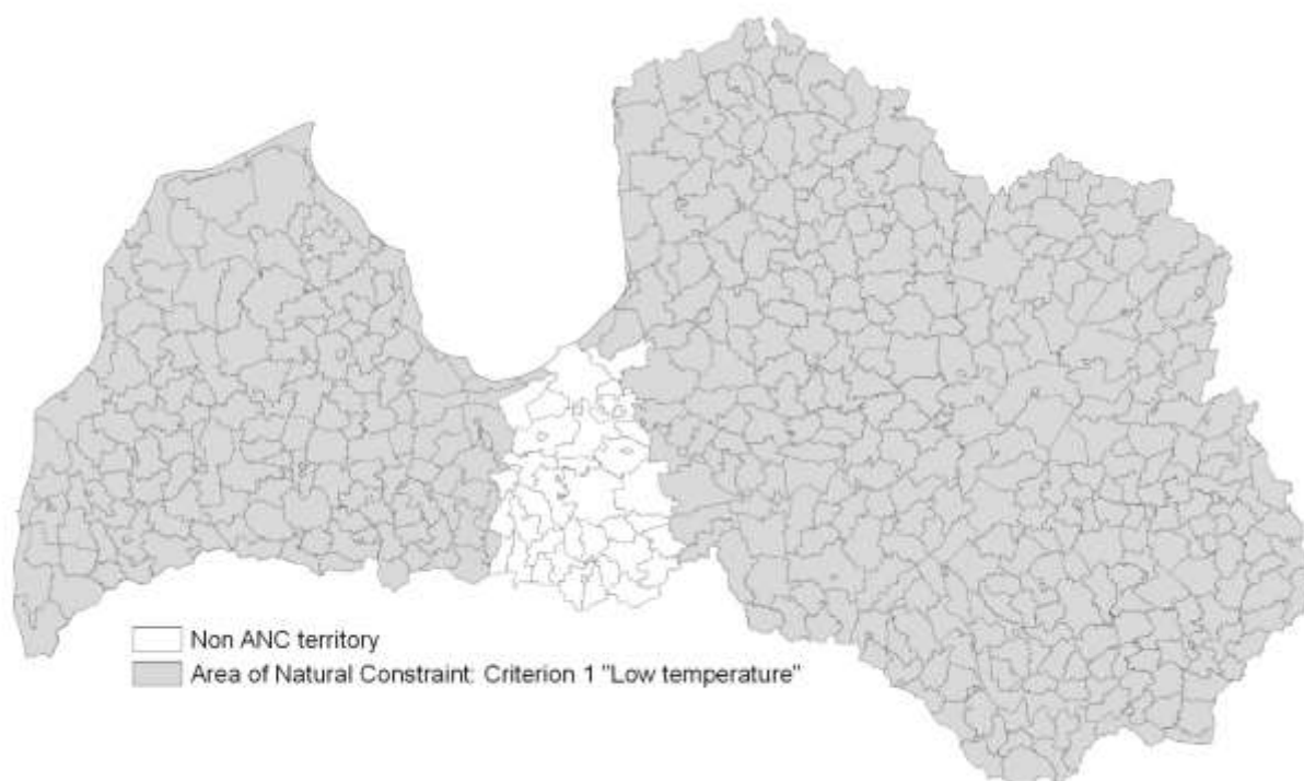
Figure 3.1-12: Delineation of ANC territories where the Thermal Time Sum ANC criterion occurrence probability exceeds 20% (8 measurement method, period 1968-2008) using co-kriging interpolation method with elevation as a secondary input variable. ANC size – 60.09 thousand km 2 or 93.08% of the total country area.
