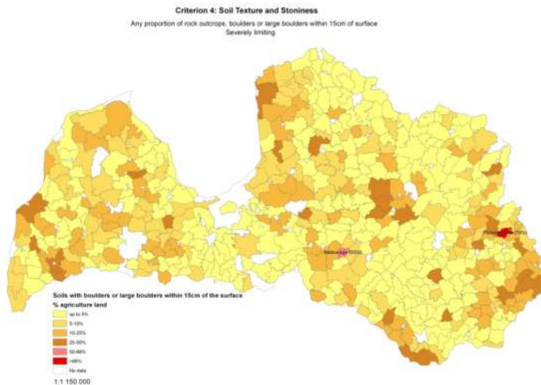
Figure 3.4-1: Overall situation in Latvia: Simulation results of the Criterion "SOIL TEXTURE AND STONINESS" - Soils where any proportion of rock outcrops, boulders within 15 cm of the surface
