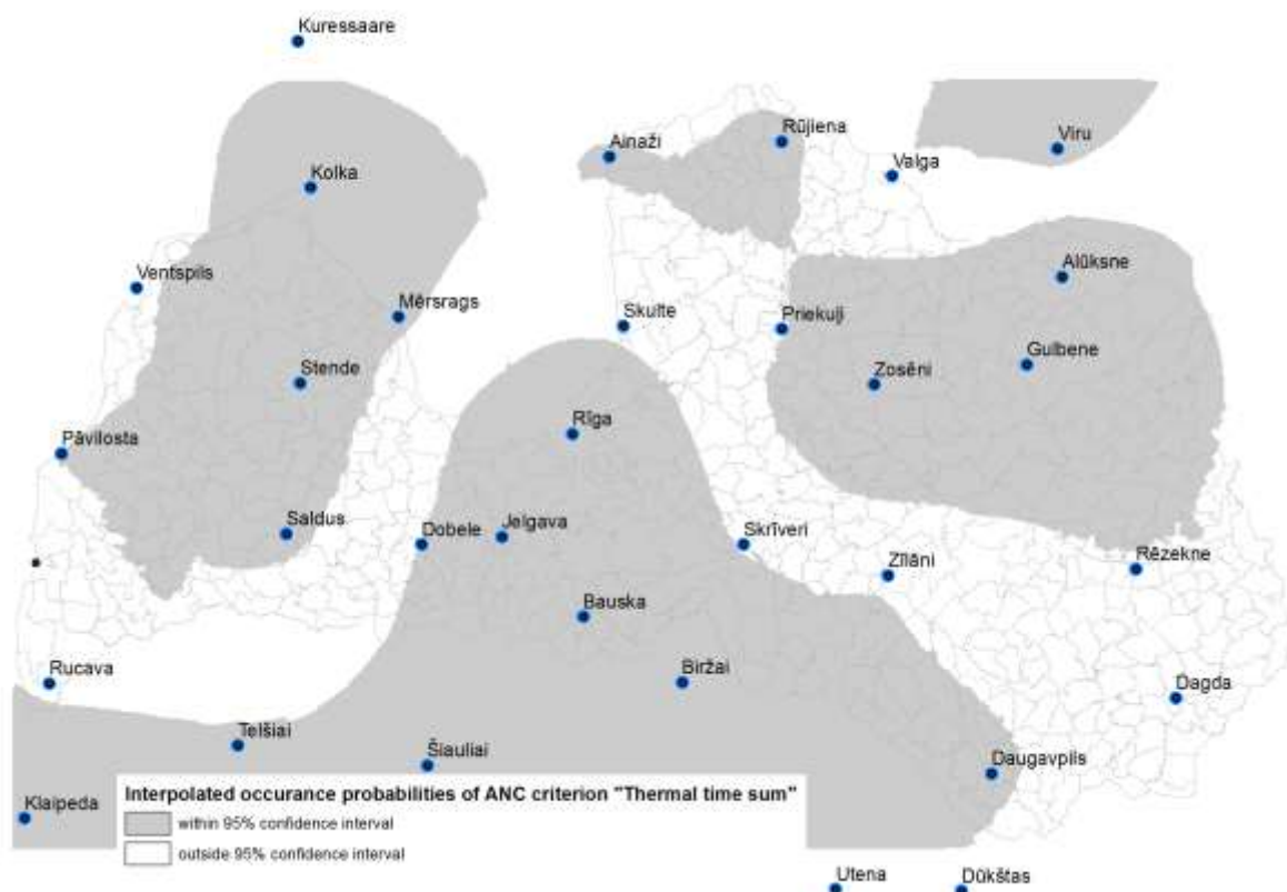
Figure 3.1-9: Interpolated occurrence probabilities of ANC criterion “Thermal time sum”
