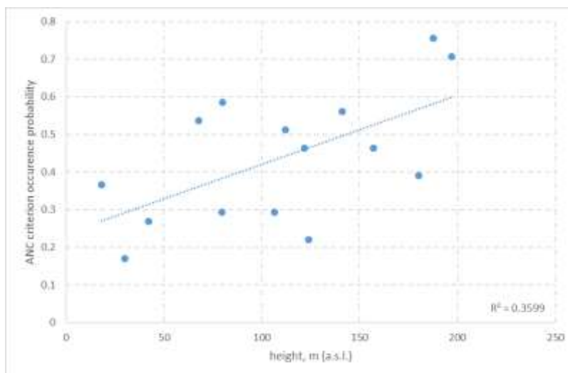
Figure 3.1-6: Relationship of ANC criterion occurrence probability vs relief, elevation (height above sea level). Statistics: Pearson r = 0.599 , r^2=0.36 , p = 0.018
