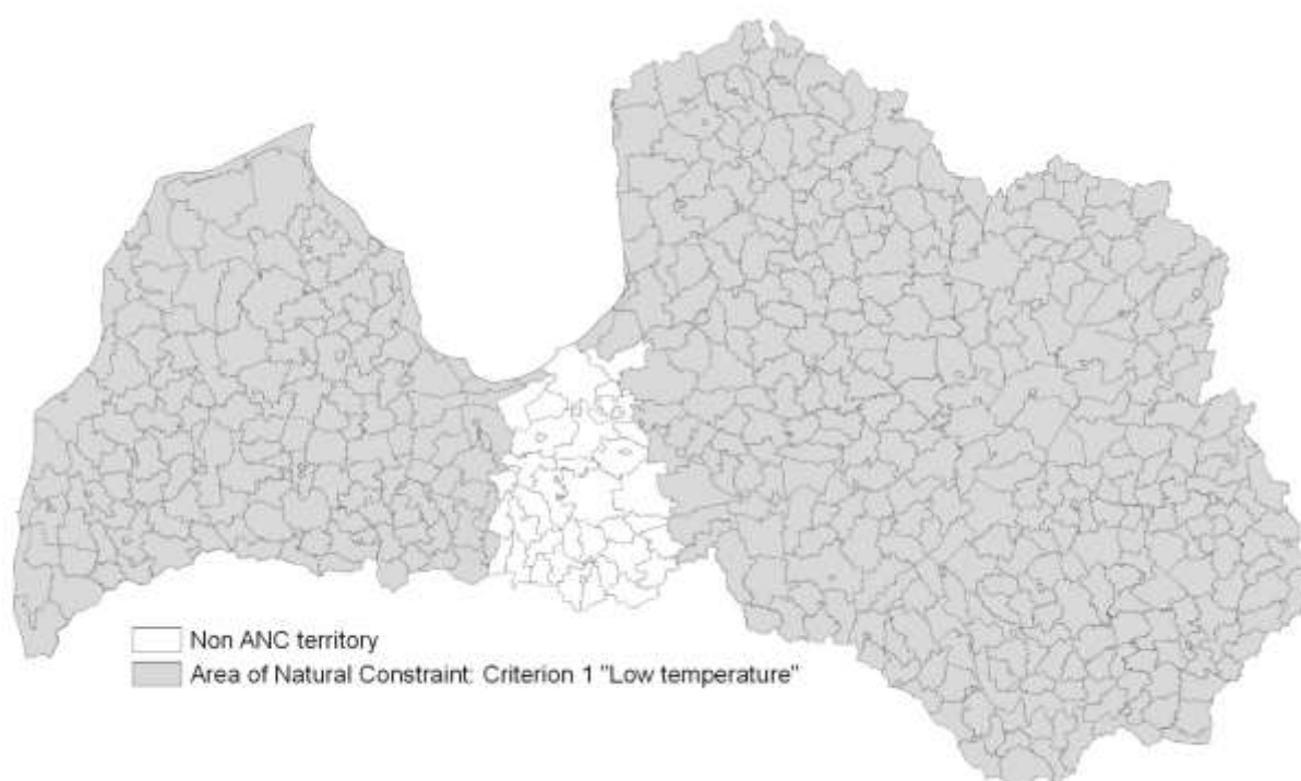
Figure 1.2-2: Territories where the thermal-time sums is ANC criterion occurrence possibility >20% (8 measurement method, period 1968-2008) on the map of territorial units with soil results.
