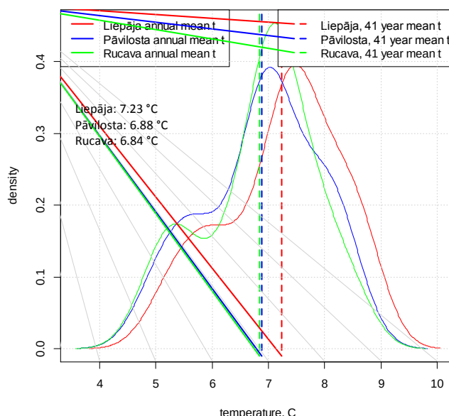
Figure 3.1-4: Comparison of annual mean temperature data sets – Liepāja, Rucava and Pāvilosta meteostations (time series data 1968-2008)
