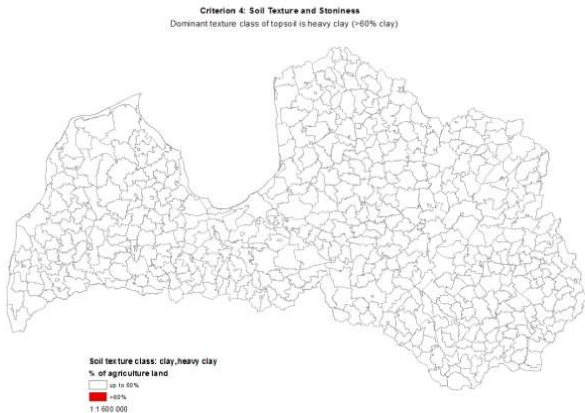
Figure 3.4-8: Criterion “SOIL TEXTURE AND STONINESS” – organic soils. Areas considered as affected by significant natural handicaps with >60% compliance
