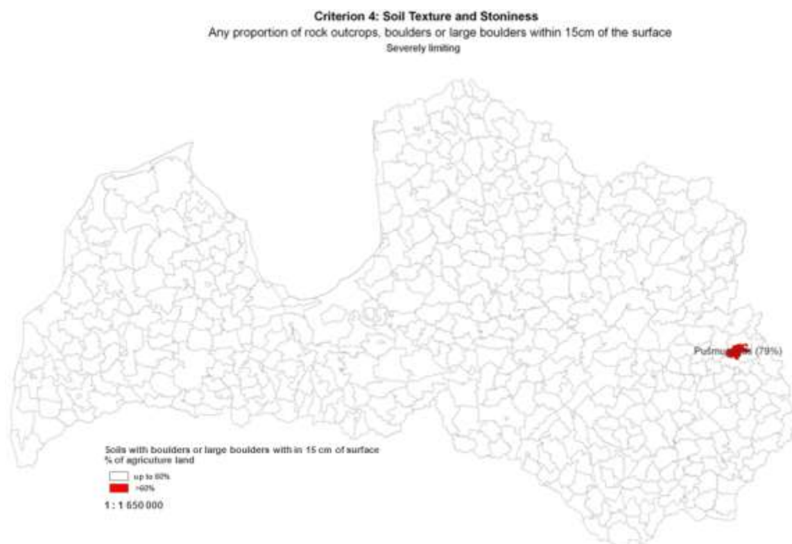
Figure 3.4-2: Criterion “SOIL TEXTURE AND STONINESS” - Soils where any proportion of rock outcrops, boulders within 15 cm of the surface. Areas considered as affected by significant natural handicaps with >60% compliance
