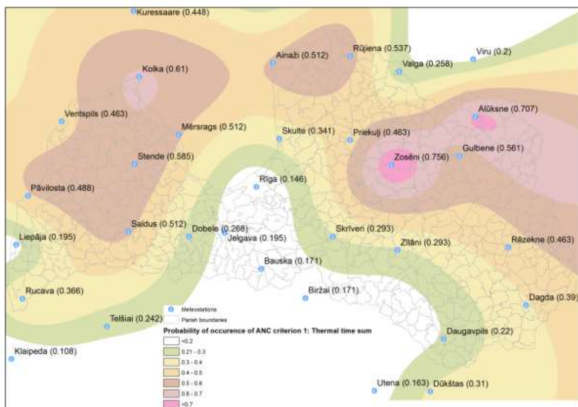
Figure 3.1-2: Delineation of ANC criterion Thermal Time Sum occurrence probabilities (8 measurement method, data range 1968-2008).
